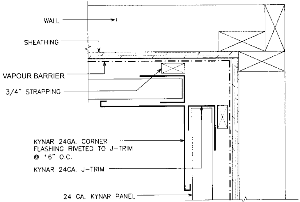
PLAN VIEW
